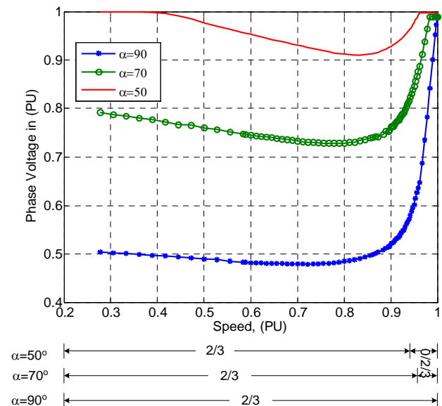
Fig.11 Phase voltage for different values of firing angle.
