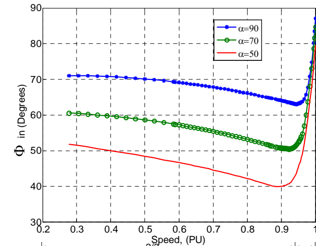
Fig. 13 Power factor variation for different values of firing angle.
